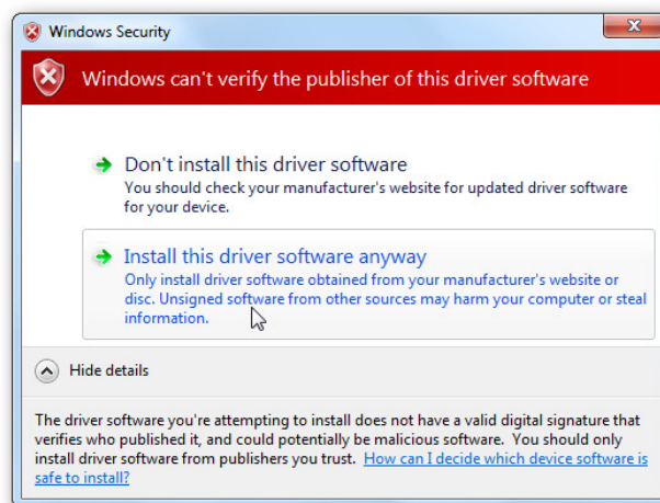
Fig 4: Windows Security
