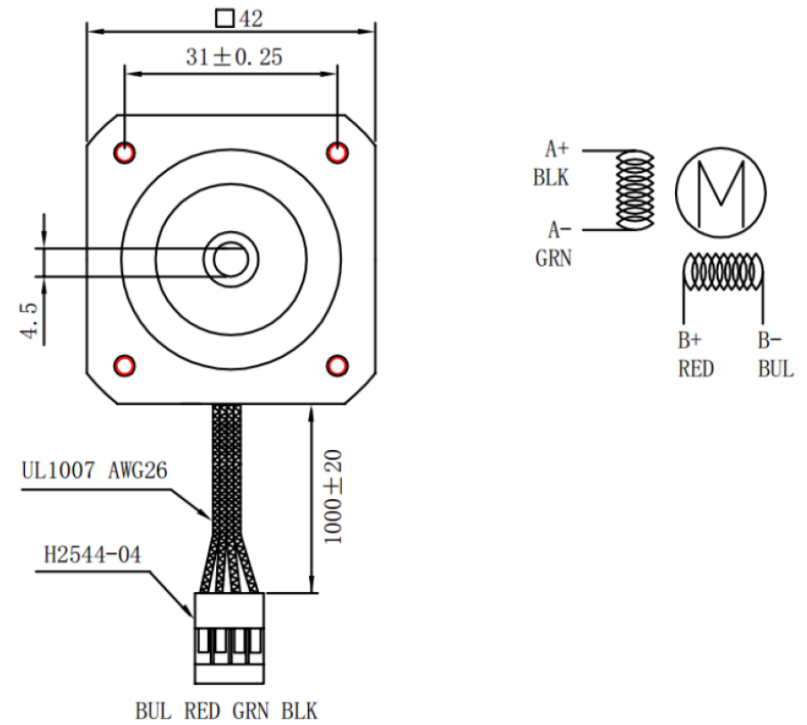
Wiring Diagram
