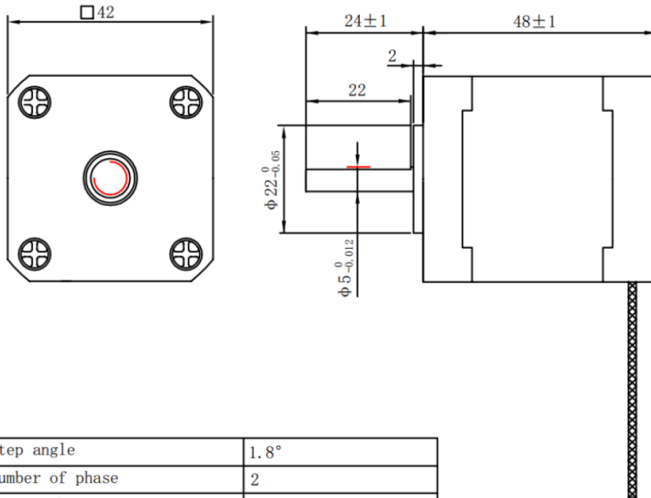
Dimensional drawing
